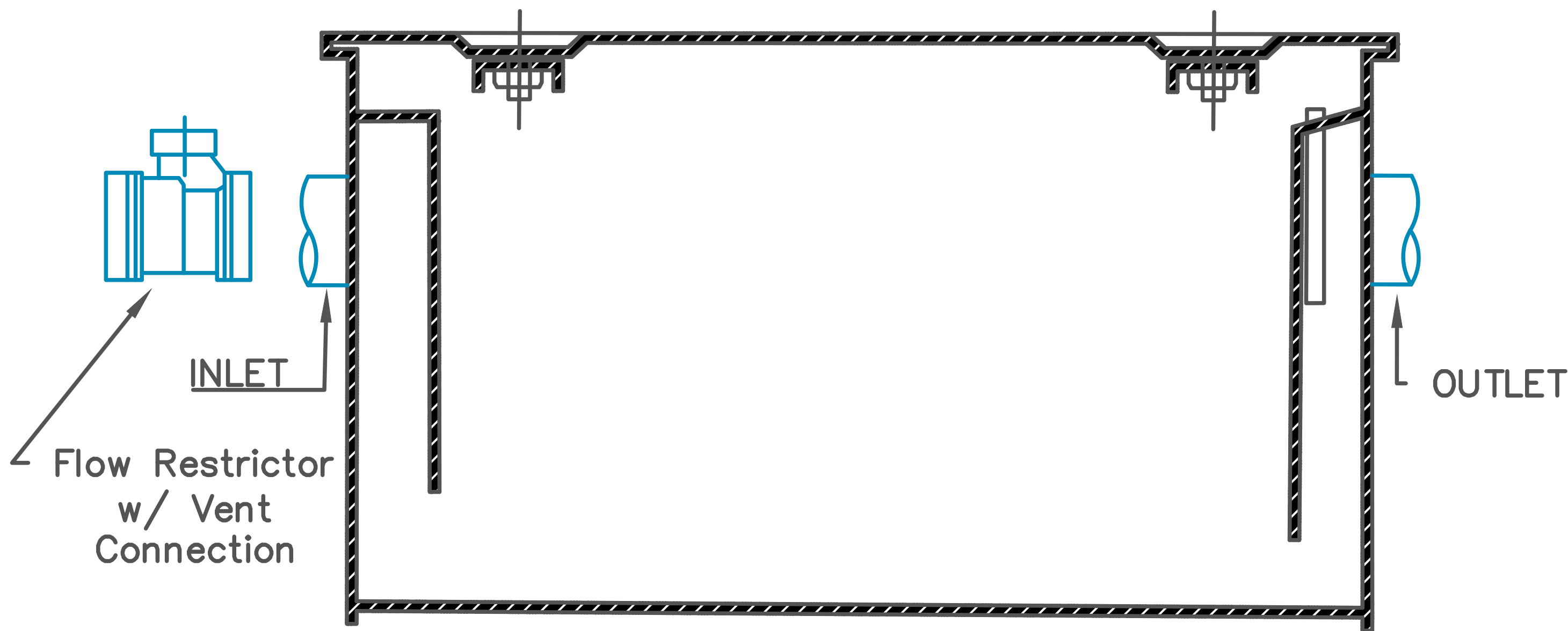
INDOOR GREASE INTERCEPTOR
