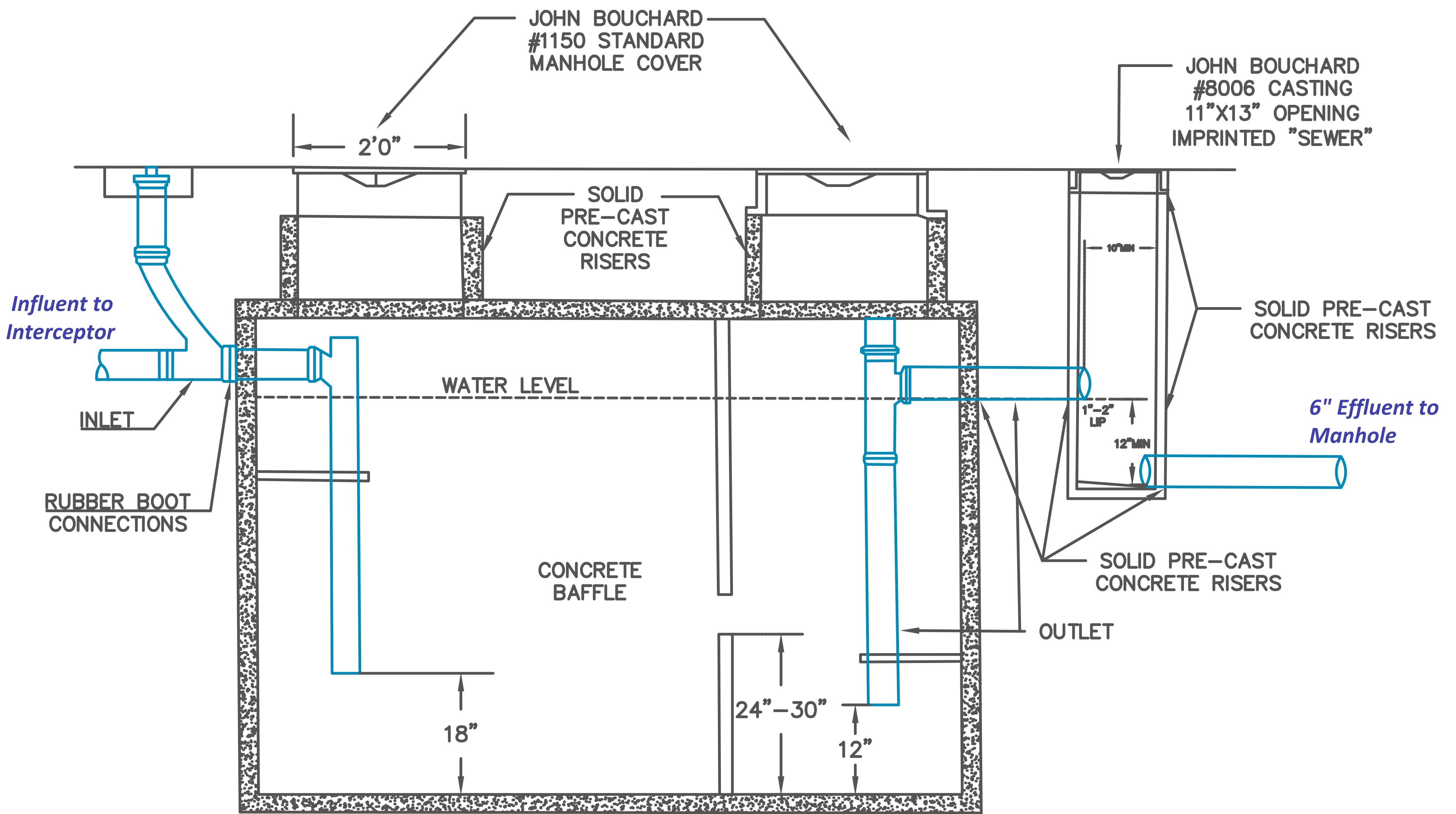
OUTDOOR GREASE INTERCEPTOR
