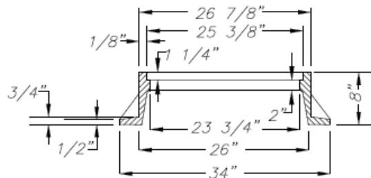
FRAME SECTION
