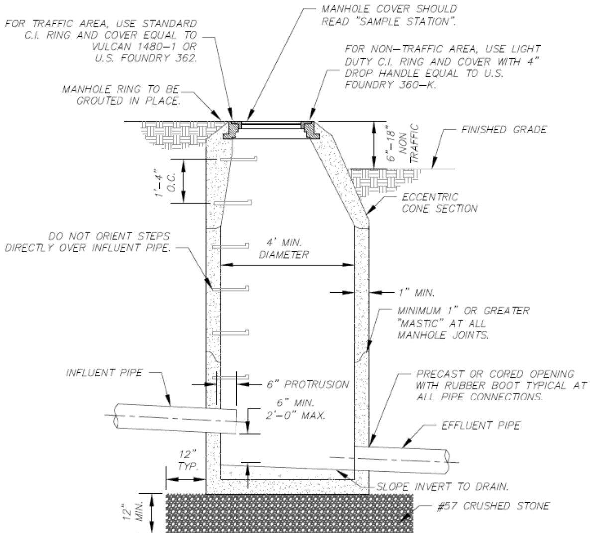
Industrial Sample Manhole NTS
