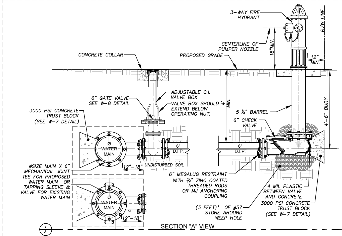
Fire Hydrant Assembled, 6" Check Valve, 6" DIP branch and 6" Gate Valve
