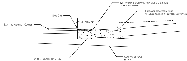
PROFILE VIEW
