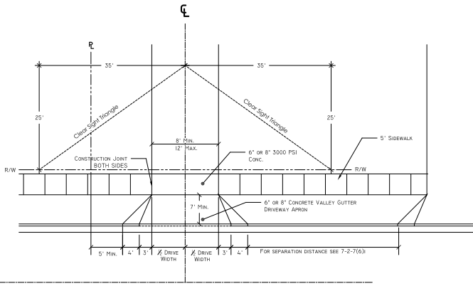
PLAN VIEW
