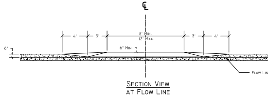
RECESSED CURB
