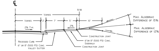
PROFILE VIEW
