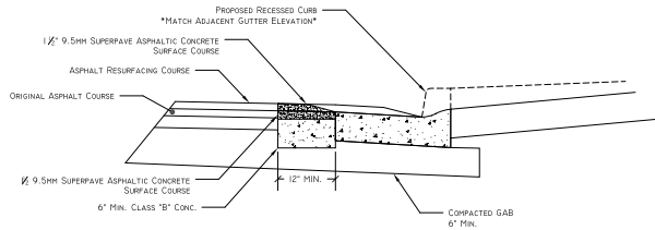
PROFILE VIEW
