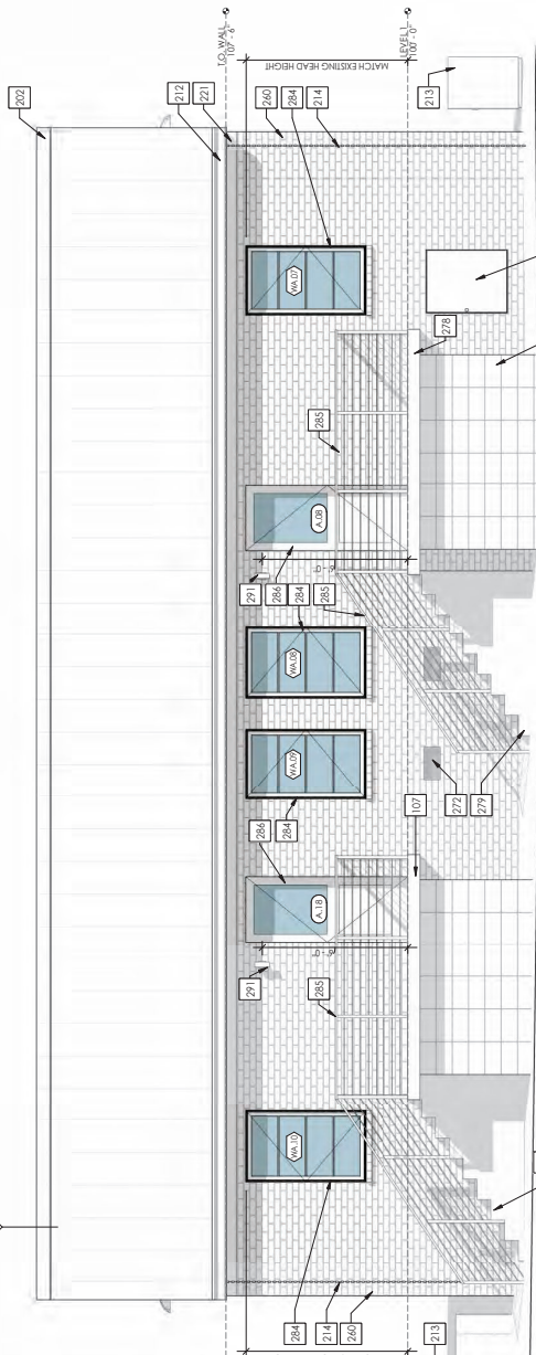
01 BUILDING A - EAST ELEVATION 1/4" = 1'-0"
