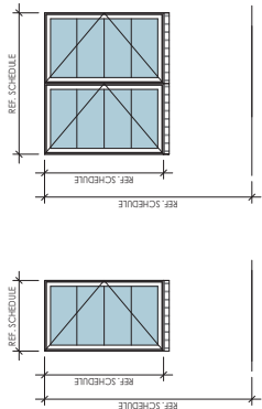
A SINGLE-VENT PELLA ARCHITECT SERIES TRADITIONAL CASEMENT B DOUBLE-VENT PELLA ARCHITECT SERIES TRADITIONAL CASEMENT
