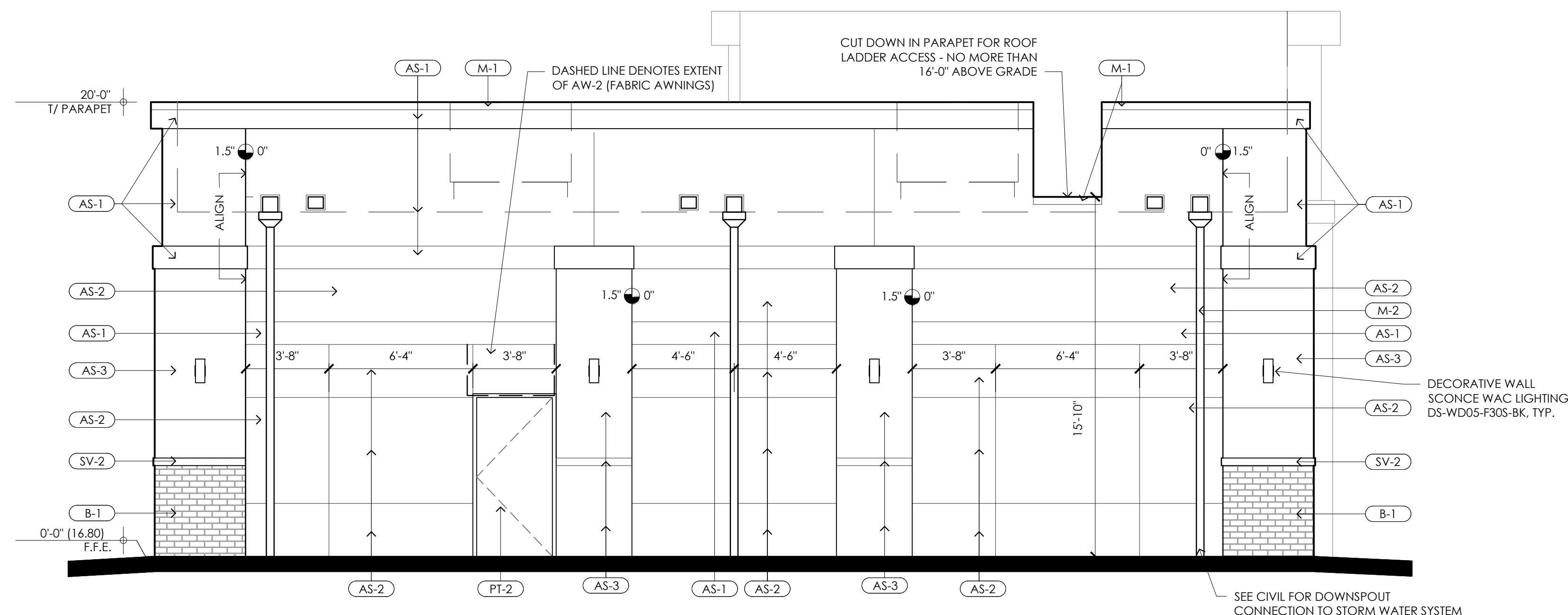
01 NORTH (REAR) ELEVATION A2.2 SCALE: 1/4" = 1'-0"
